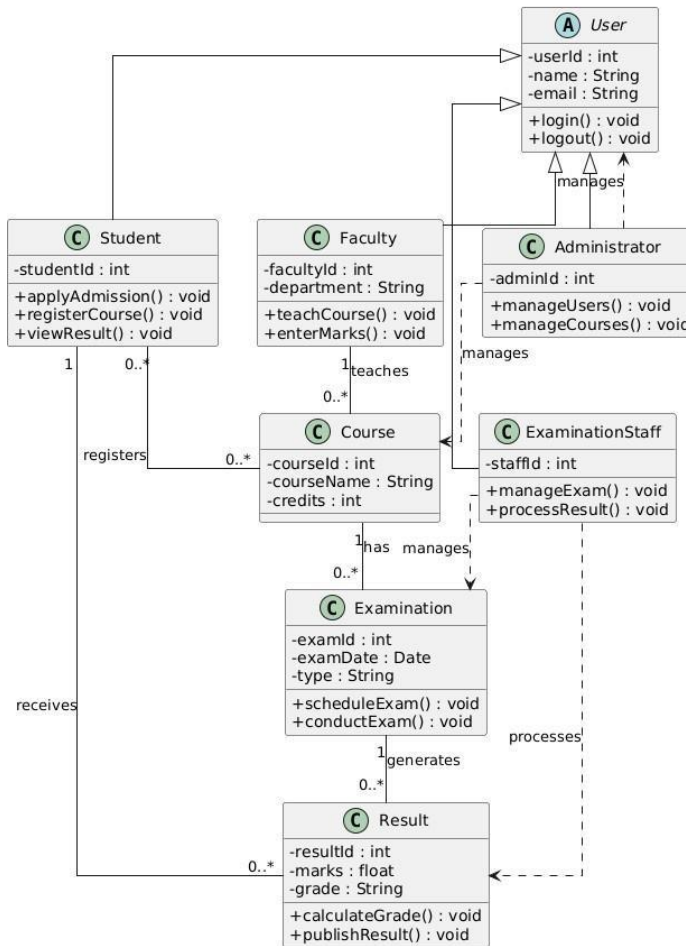
University Management System - Class Diagram
